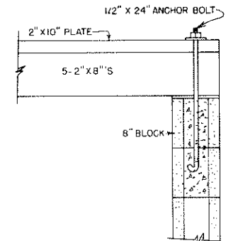
DETAIL OF INSIDE END OF GIRDER
