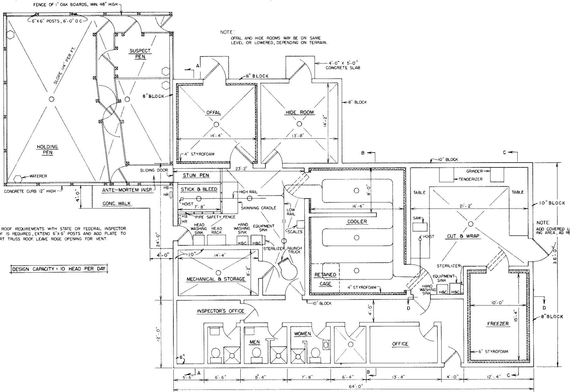
FLOOR PLAN
