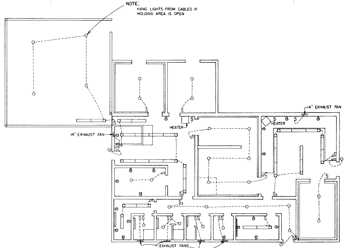
ELECTRICAL LAYOUT
