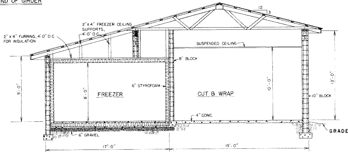
SECTION C-C
