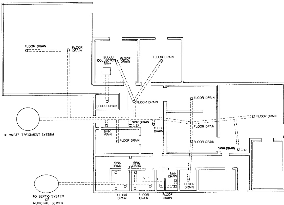
DRAIN SYSTEMS
