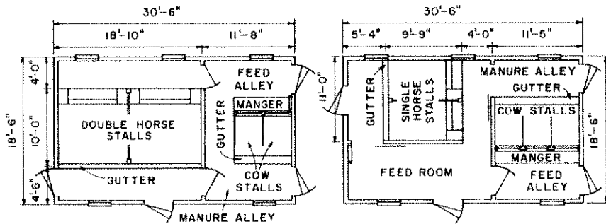
ALTERNATE PLANS
