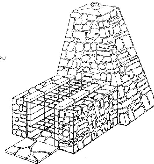
PERSPECTIVE
