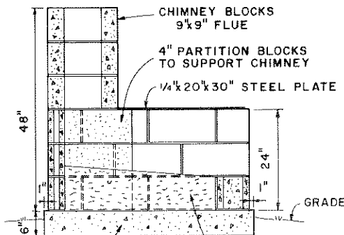
SECTION
