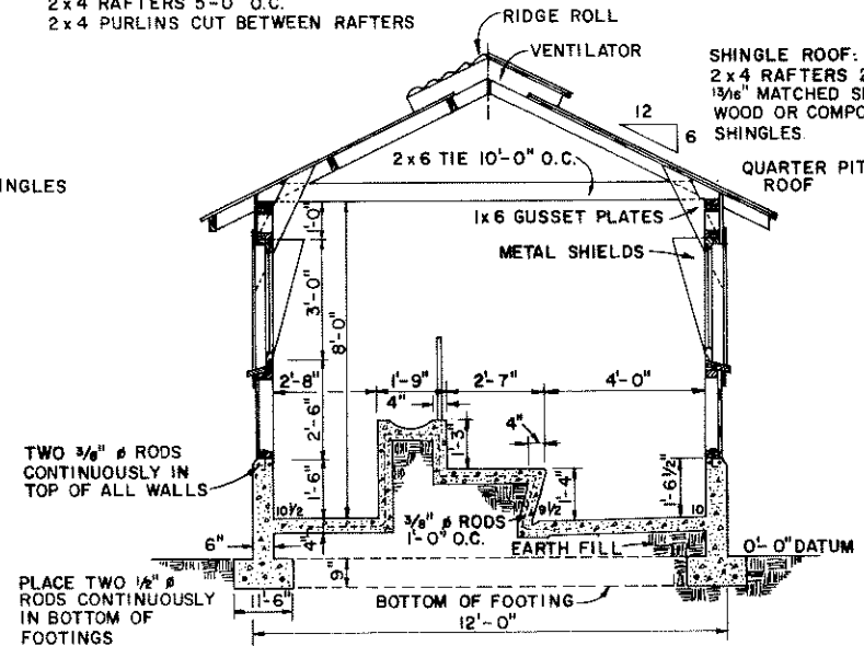
SECTION "B-B"
