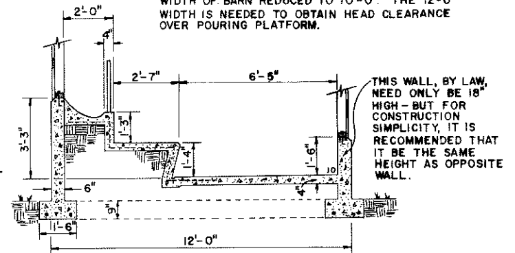
ALTERNATE SECTION "B-B"
