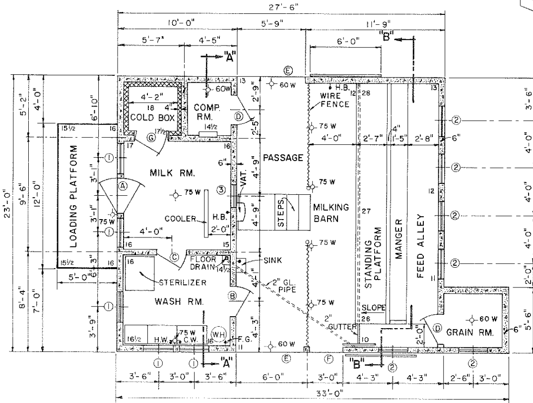
FLOOR PLAN
