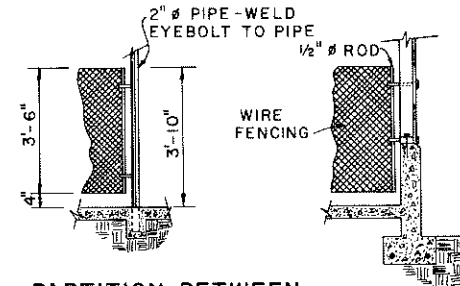
DETAIL - PARTITION BETWEEN MILKING BARN & PASSAGE
