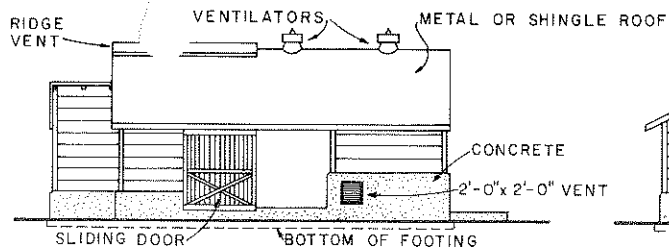
NORTH ELEVATION
