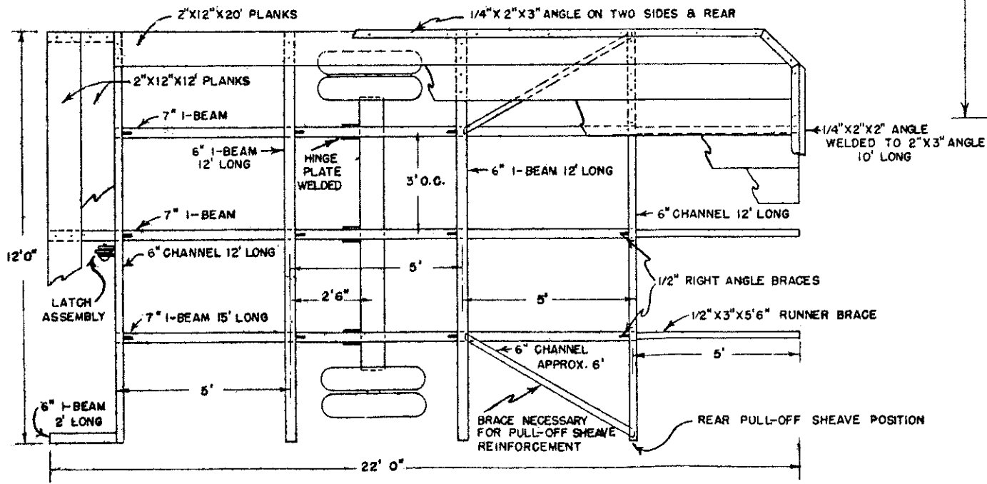
TOP VIEW BED STRUCTURE
