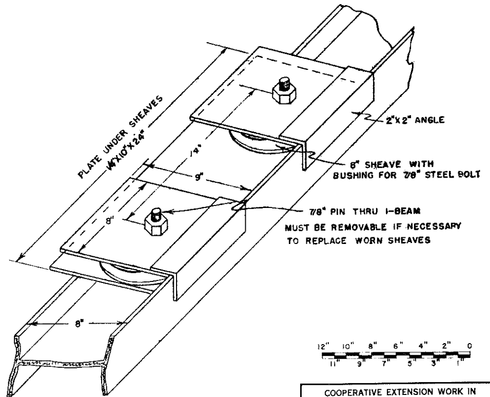
CENTER OF PULL-ON BEAM
