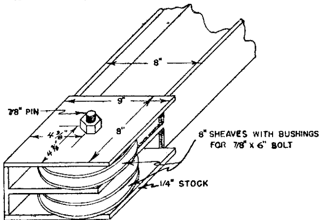
END OF PULL-ON BEAM
