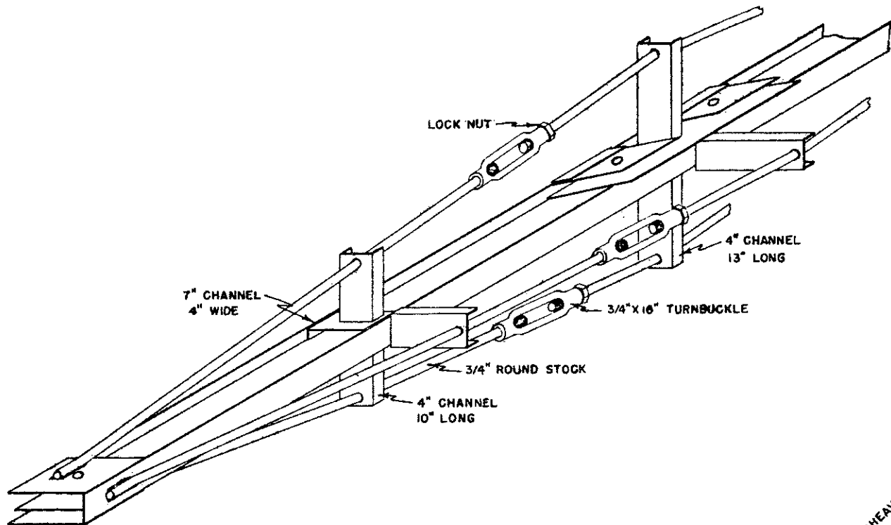
PULL-ON BEAM BRACING SCALE: 1 1/2" = 1'
