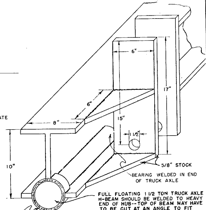
PIN ASSEMBLY DETAIL
