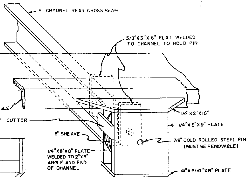
REAR PULL-OFF SHEAVE DETAIL
