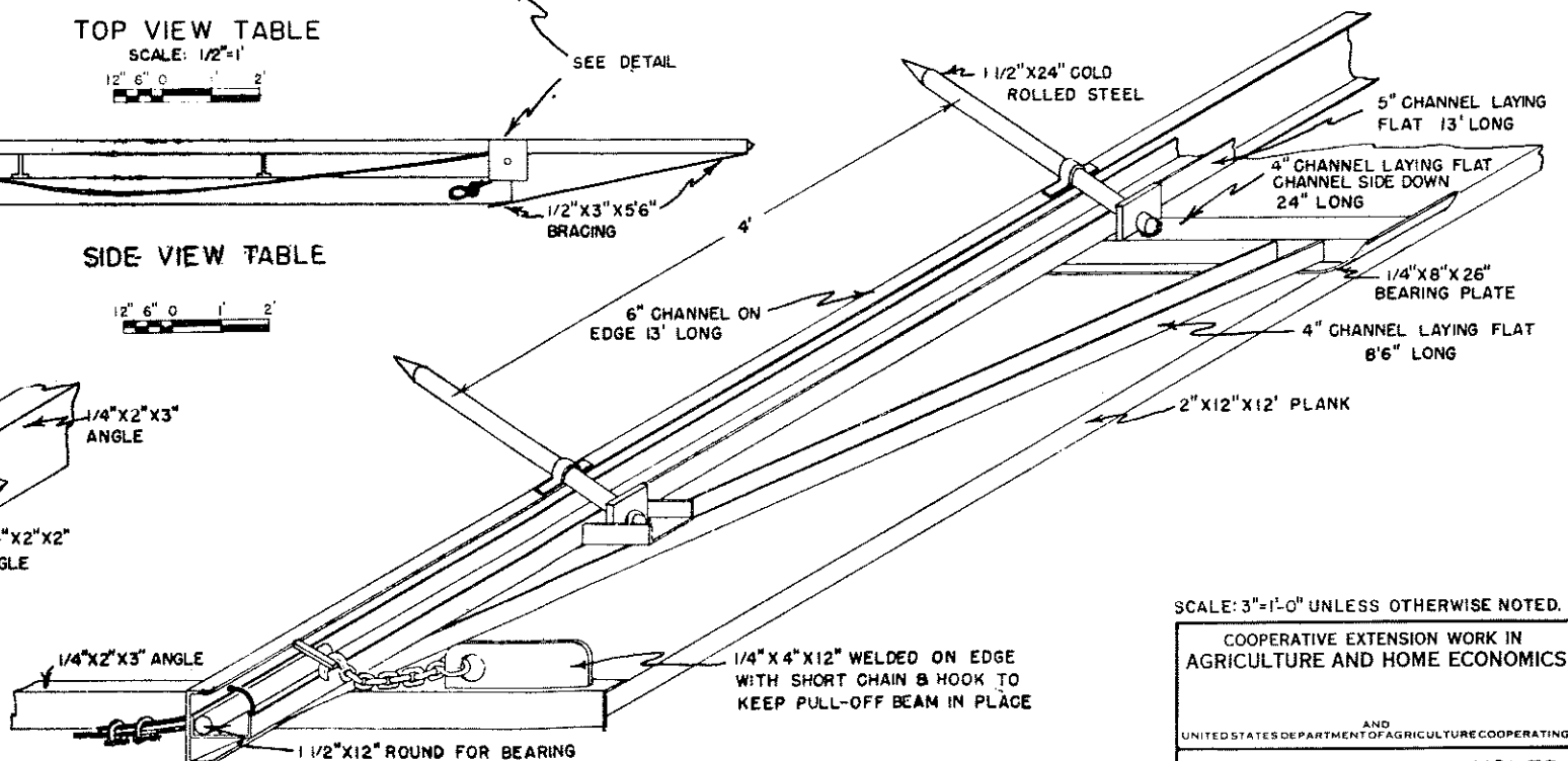
PULL-OFF BEAM DETAIL
