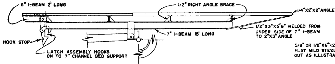
SIDE VIEW BED STRUCTURE
