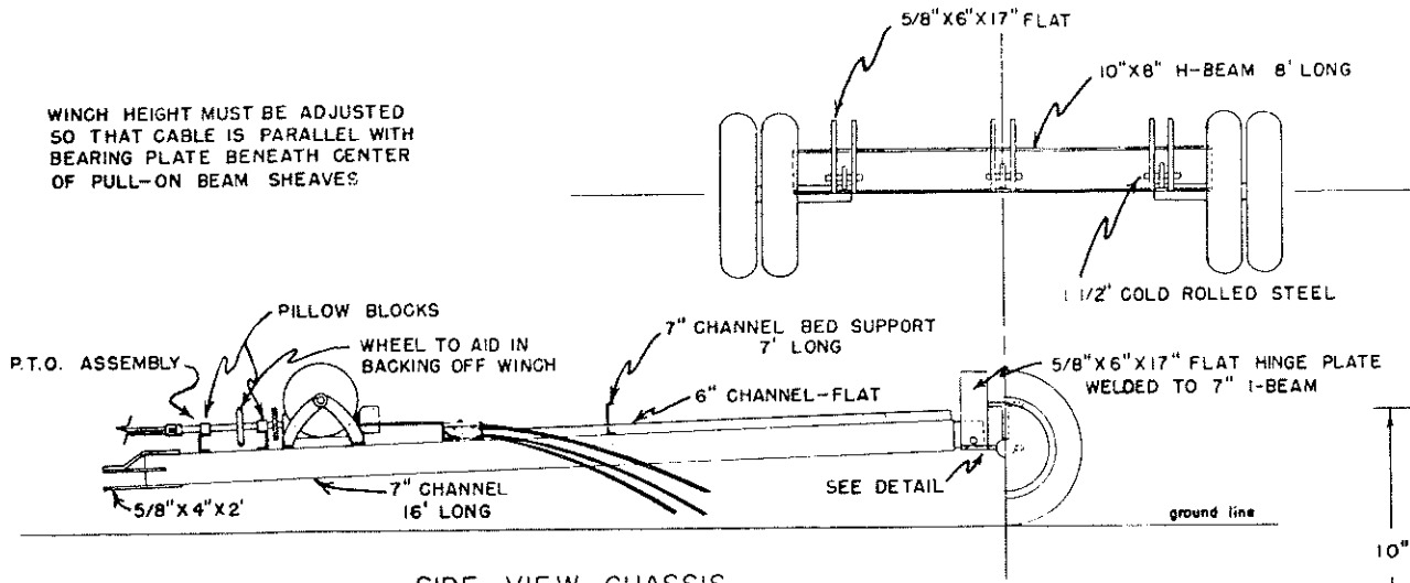
SIDE VIEW CHASSIS
