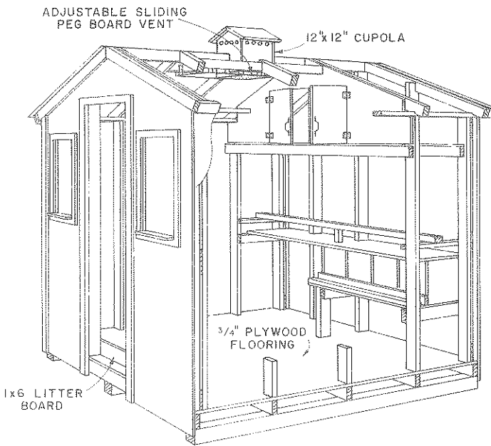
CUTAWAY VIEW OF 8x8' LAYING HOUSE
