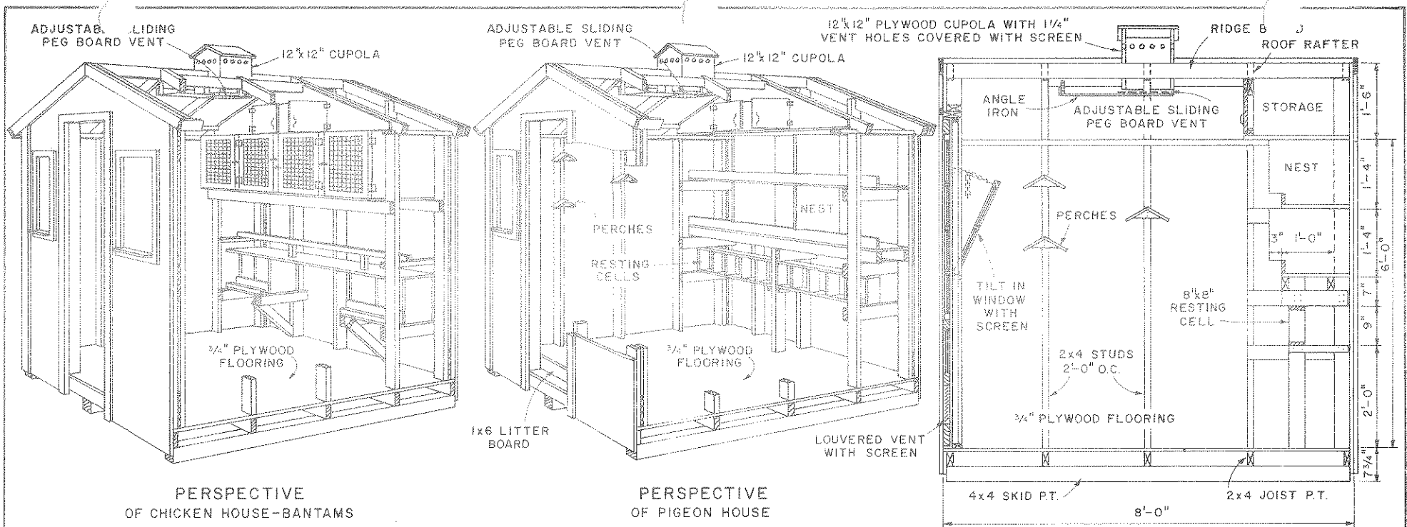
SECTION OF PIGEON HOUSE
