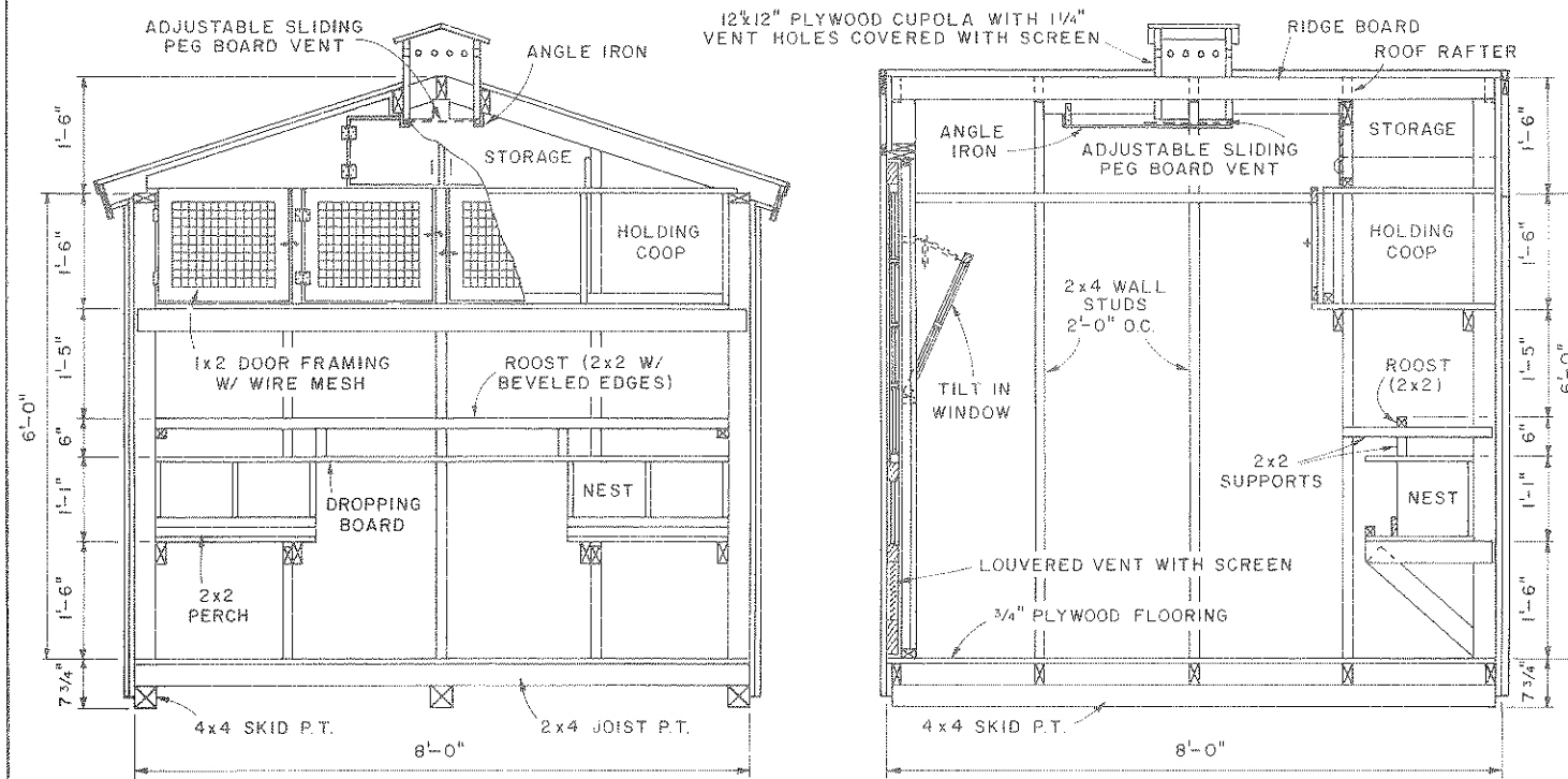
SECTIONS OF CHICKEN HOUSE-BANTAMS
