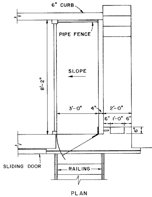
KNOCKING PEN DETAILS
