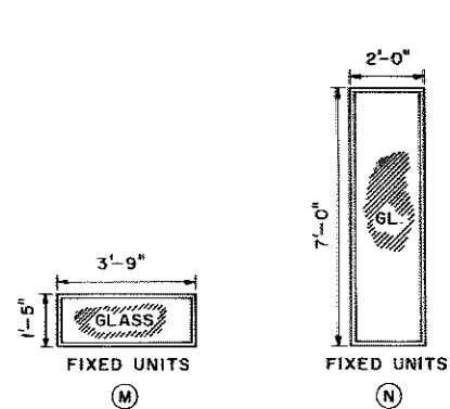
WINDOW SCHEDULE
