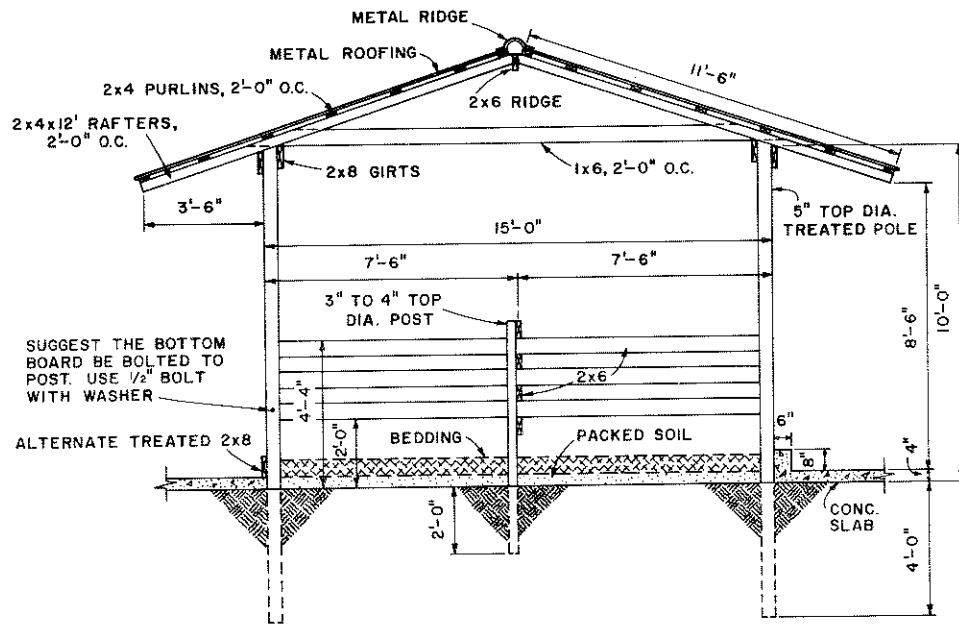
SECTION "B-B" DOUBLE STALL BARN
