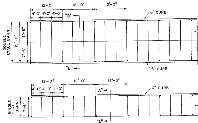
PLAN-SINGLE AND DOUBLE STALL BARN
