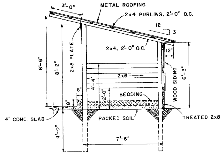
SECTION "A-A" SINGLE STALL BARN
