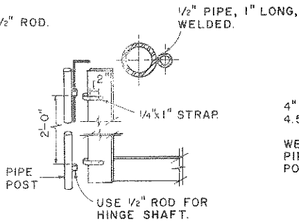
HINGES NOT TO SCALE
