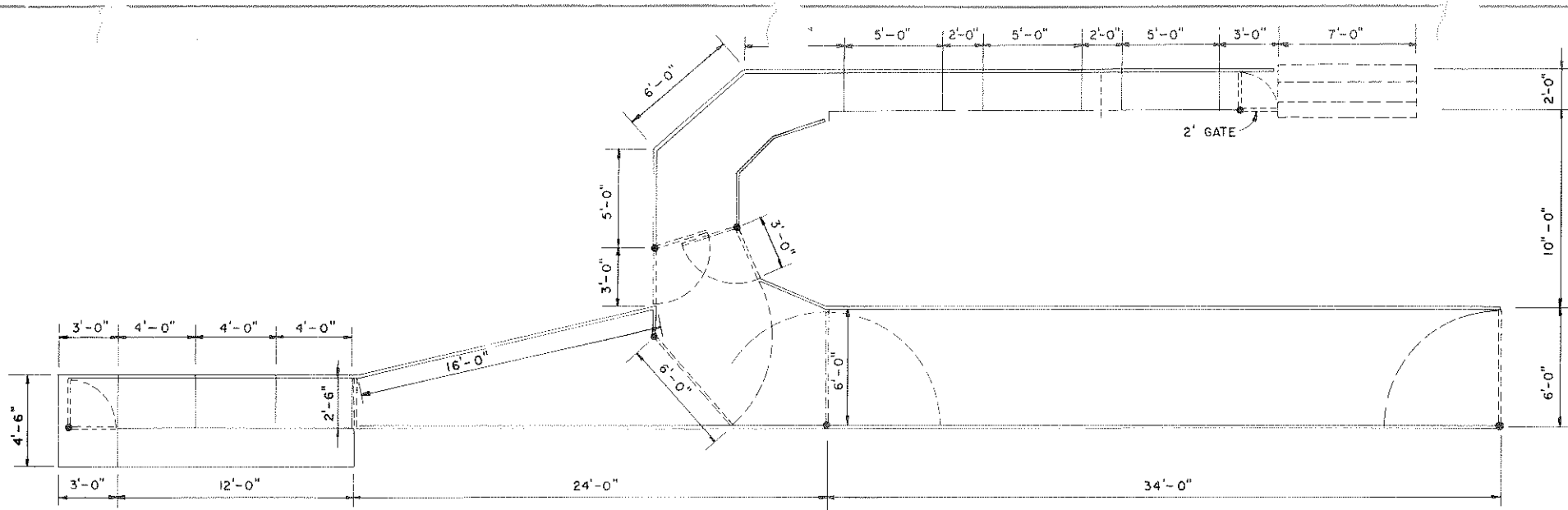
PLAN SCALE: 1/4" = 1'-0" 12' 0" 2' 3' 4'
