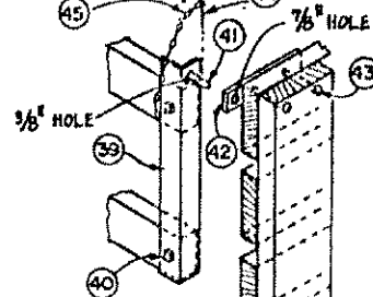
FRONT PLATFORM LATCH
