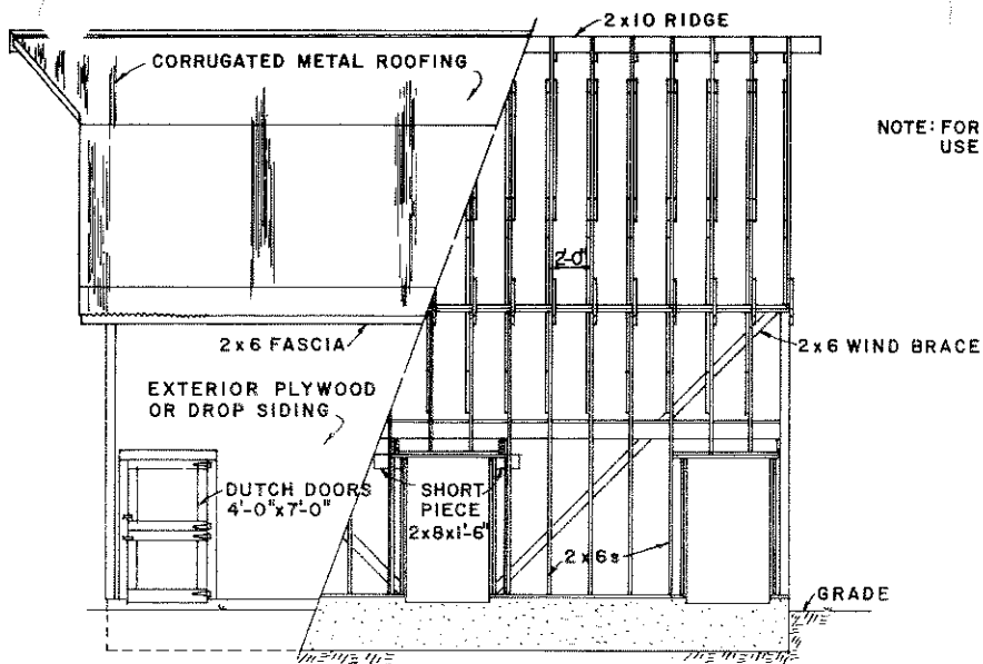
PARTIAL FRAMING-SIDE ELEVATION
