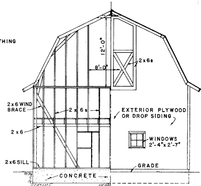
PARTIAL FRAMING-END ELEVATION
