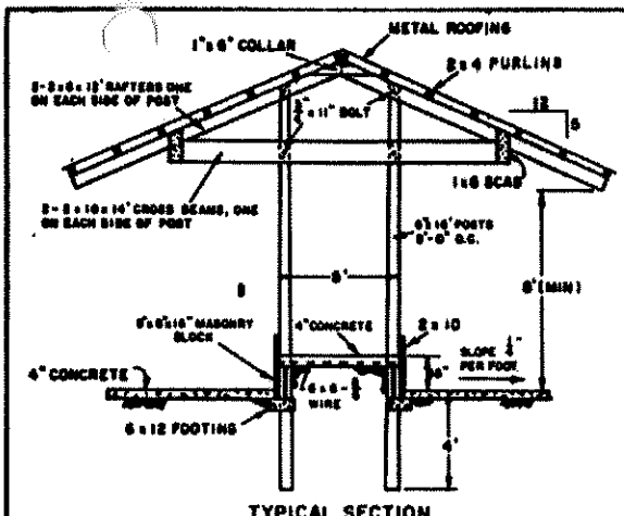
TYPICAL SECTION
