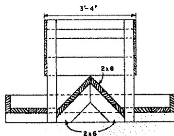
CROSS SECTION WITH CENTER DIVERTER
