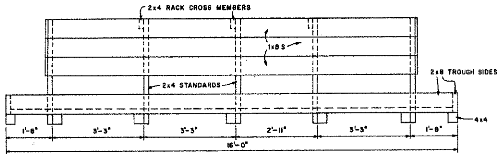
SIDE VIEW
