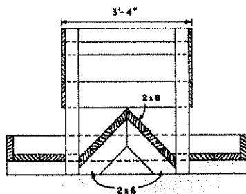
CROSS SECTION WITH CENTER DIVERTER
