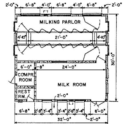
DOUBLE 6 STALL
