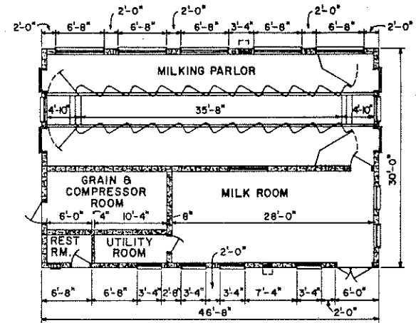
DOUBLE 10 STALL
