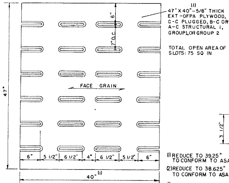
BOTTOM DETAIL *
