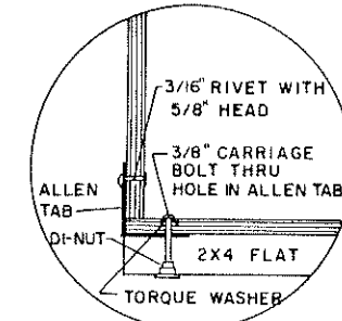
STRINGER END
