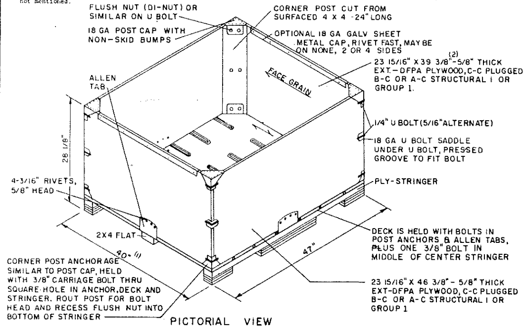
PICTORIAL VIEW
