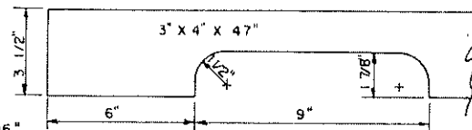
ALTERNATE STRINGER
