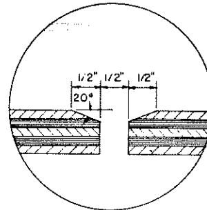
SECTION THRU SLOT *
