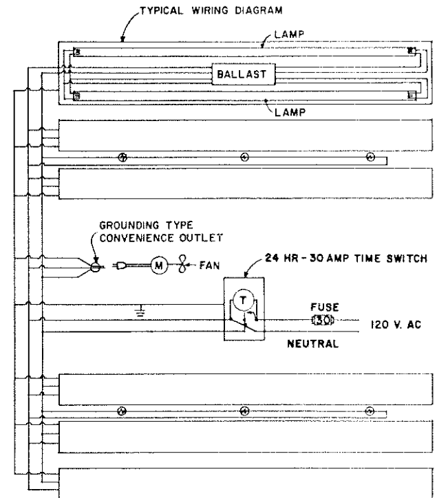
WIRING SCHEMATIC NO SCALE
