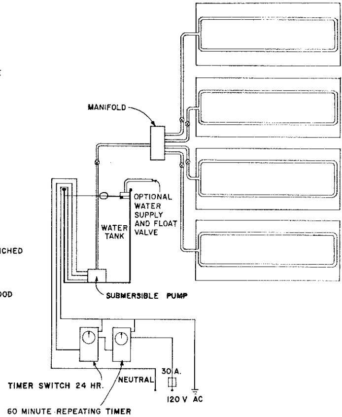
WATERING SYSTEM WITH TIME CLOCKS NO SCALE
