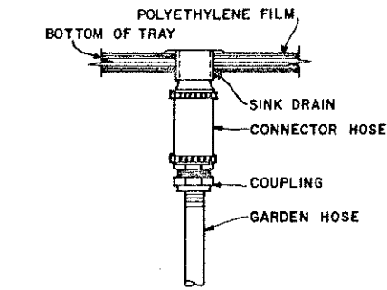
DETAIL OF DRAIN NO SCALE
