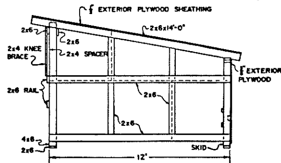
END FRAMING
