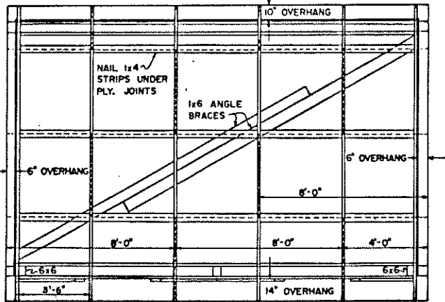
ROOF FRAMING
