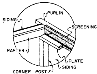
SCREENING DETAIL
