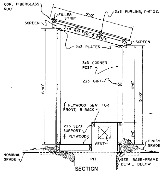
SECTION
