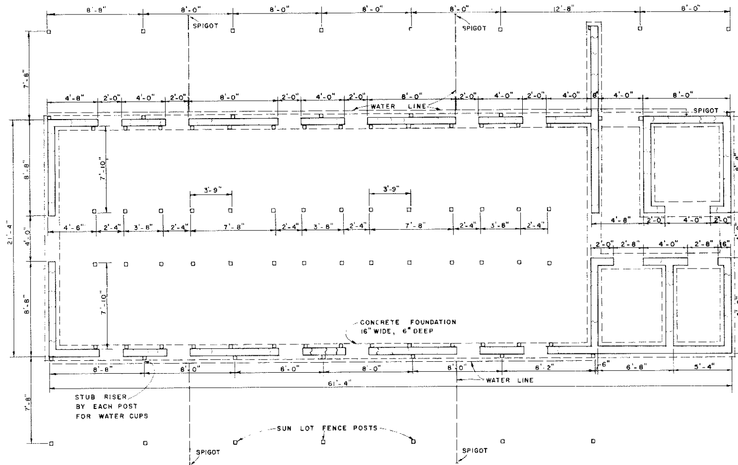
POST & FOUNDATION PLAN
