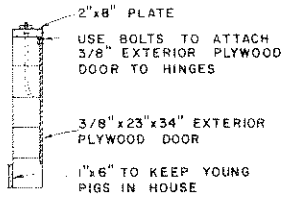
SIDE ELEVATION 0 4 8 12 FT.
