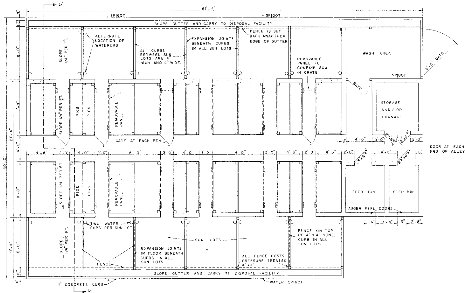
FLOOR PLAN SCALE: 0 2 4 6 FT.
