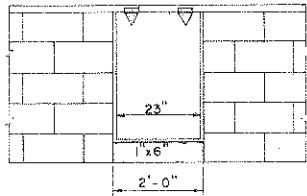
SUN LOT ACCESS DOOR DETAILS SCALE: 0 1 2 3 FT.
