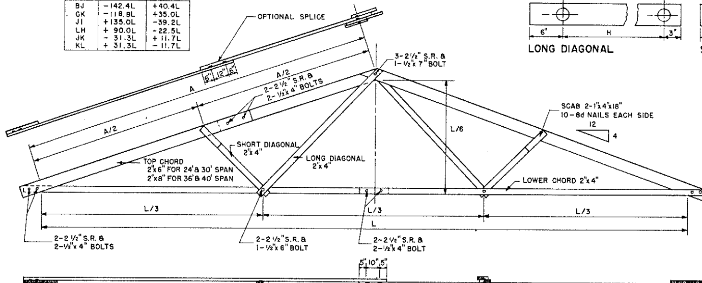
TRUSS ELEVATION
