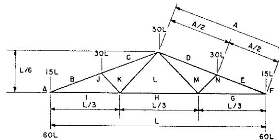
LOADING DIAGRAM
