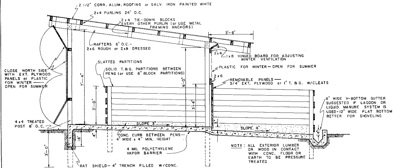
CROSS SECTION
