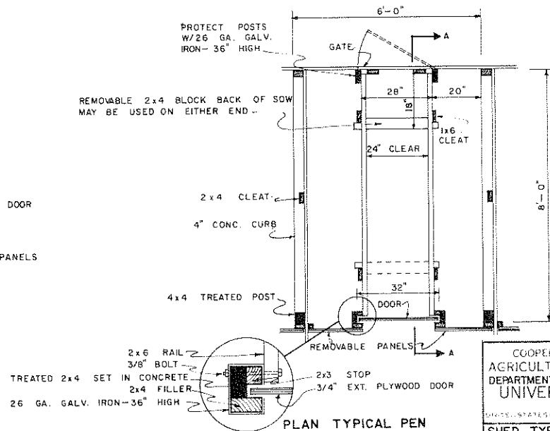
PLAN TYPICAL PEN SCALE: 0 1 2 3 FT.
