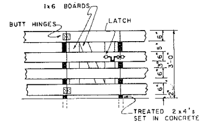
GATE & FENCE DETAIL
