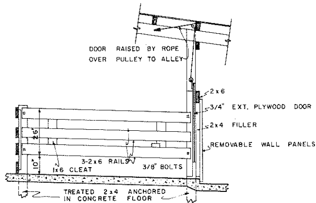
SECTION: A-A SCALE: 0 1 2 .3 FT.
