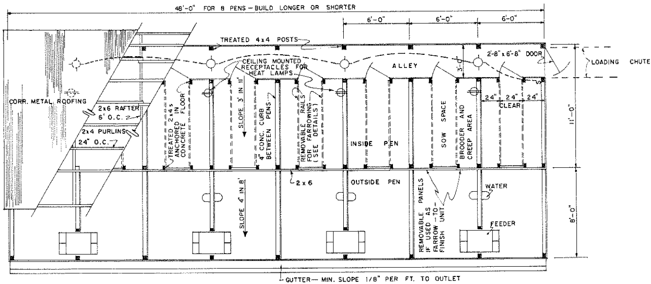
FLOOR PLAN SCALE: 0 2 4 6 FT.
