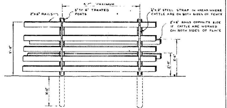
TYPICAL FENCE SCALE 0 1 2 3 4 FT.
