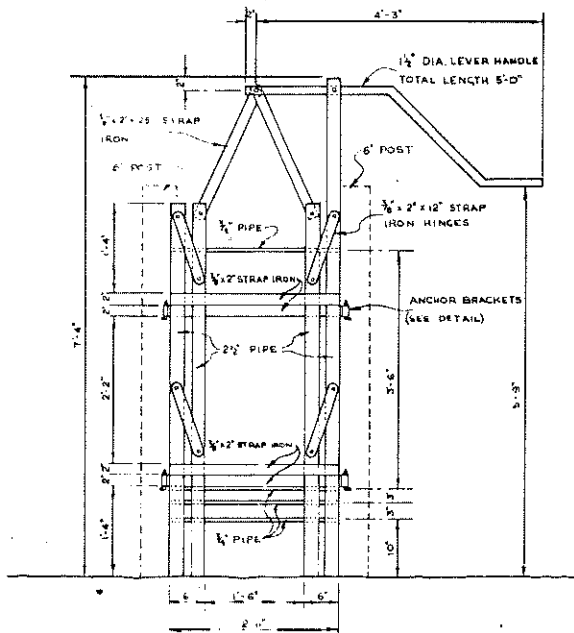
FRONT VIEW OF HEADGATE SCALE 0 1 2 FT.
