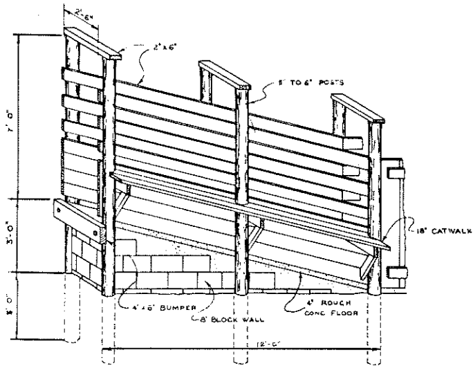
LOADING RAMP DETAIL SCALE 0 1 2 3 4 FT.
