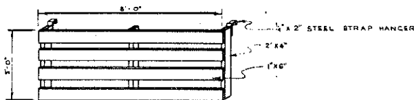
PANELS TO HANG IN CHUTE FOR WORKING SMALL CALVES SCALE 0 1 2 3 4 FT.
