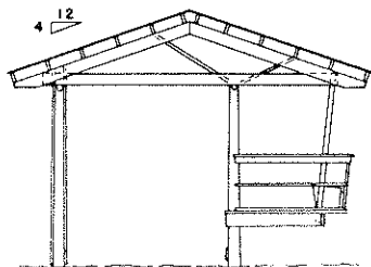
ELEVATION "A"
