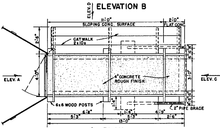
DETAILS OF LOADING RAMP SCALE: 0 1 2 3 4 FT.
