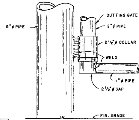
SCALE: 0 1 2 3 FT. UNLESS OTHERWISE NOTED.
