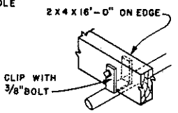
RIDGE DETAIL SCALE: 0 1 FT.
