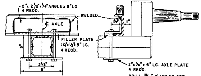
DETAIL B SCALE: 0 2 4 6 IN.
