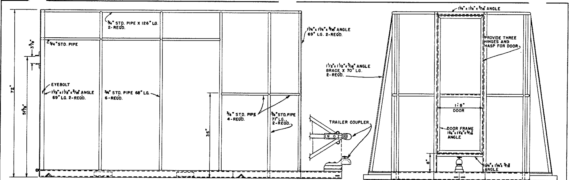
SIDE VIEW OF FRAME
