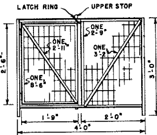
GATE END
