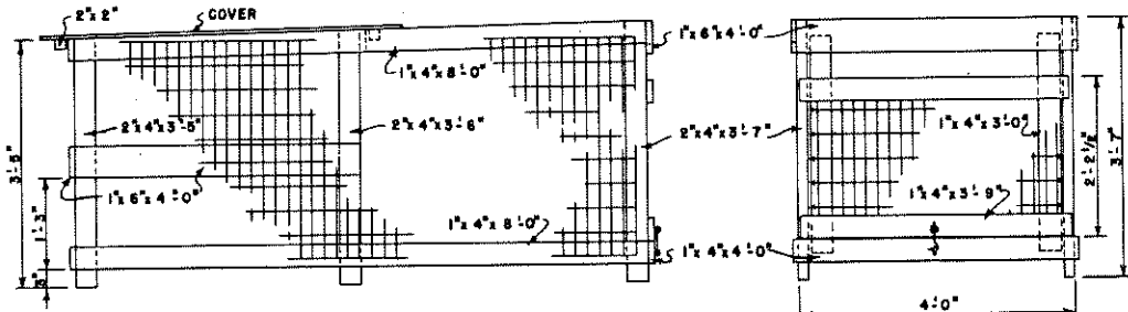
GATE END
