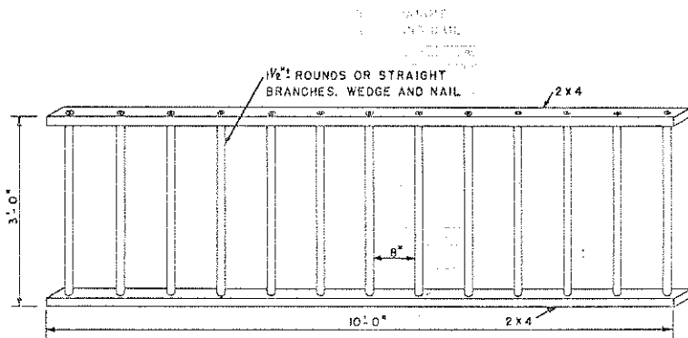
CREEP PANEL
