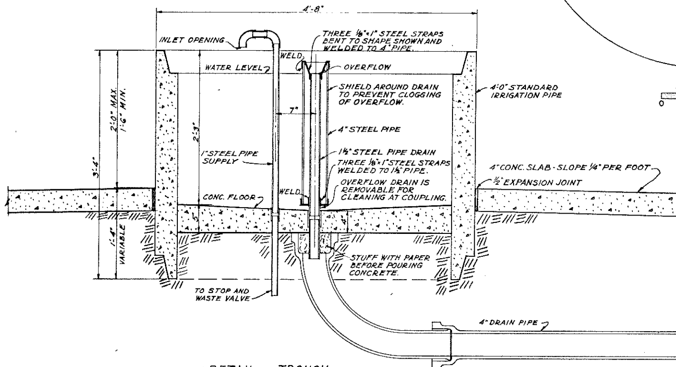
DETAIL of TROUGH 0 1 FT.
