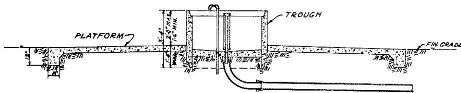
SECTION A-A 0 1 2 3 4 FT.
