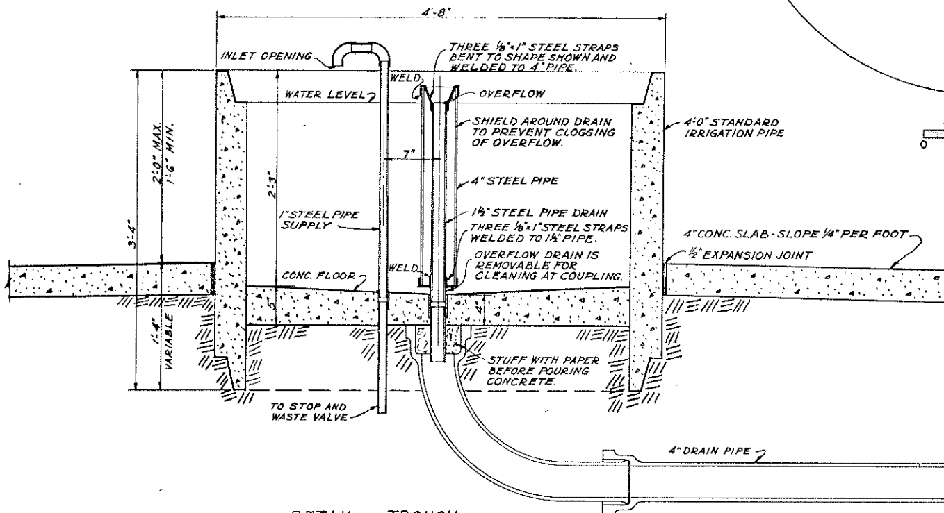
DETAIL of TROUGH
