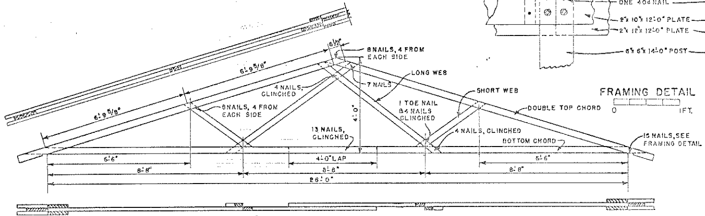
TRUSS DETAIL 0 1 2 3 FT.
