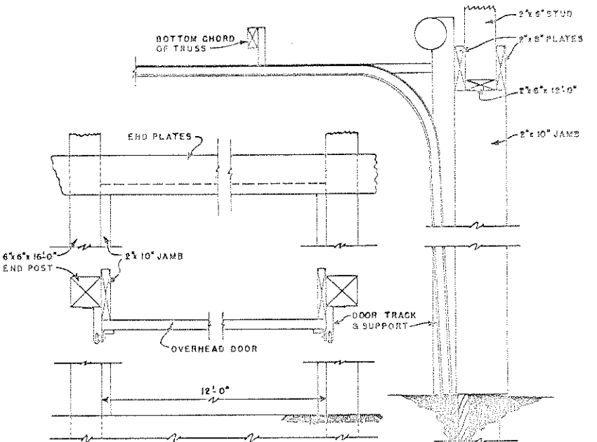
TYPICAL INSTALLATION FOR OVERHEAD DOORS SEE MANUFACTURERS DIRECTIONS FOR DETAILS
