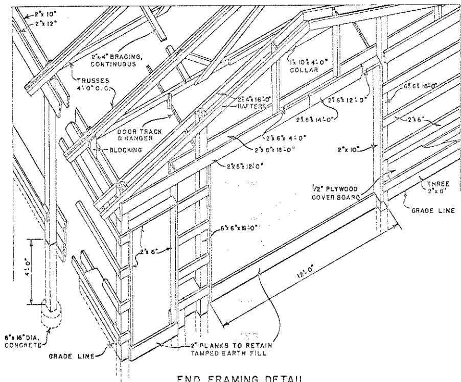
END FRAMING DETAIL 0 1 2 3 4 FT.
