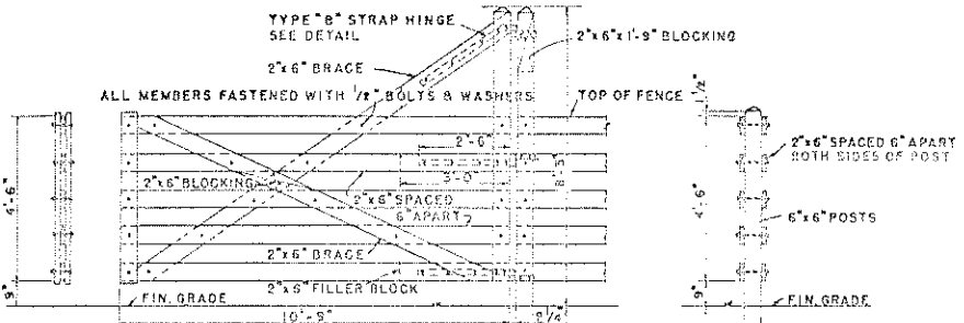
GATE AND FENCE DETAIL
