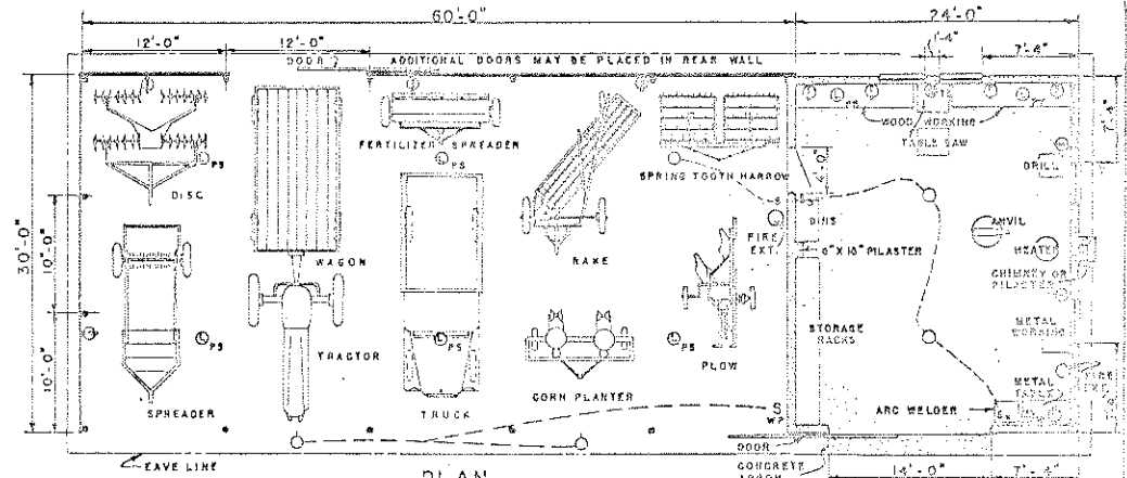
PLAN 0 4 8 12 FT.
