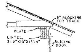
DETAIL AT LINTEL OVER SHOP DOOR
