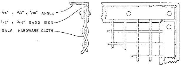
SCREEN DETAIL
