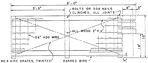
ALTERNATE PANEL CONSTRUCTION SUITABLE FOR HOT CLIMATES SCALE 0 1 2 FT
