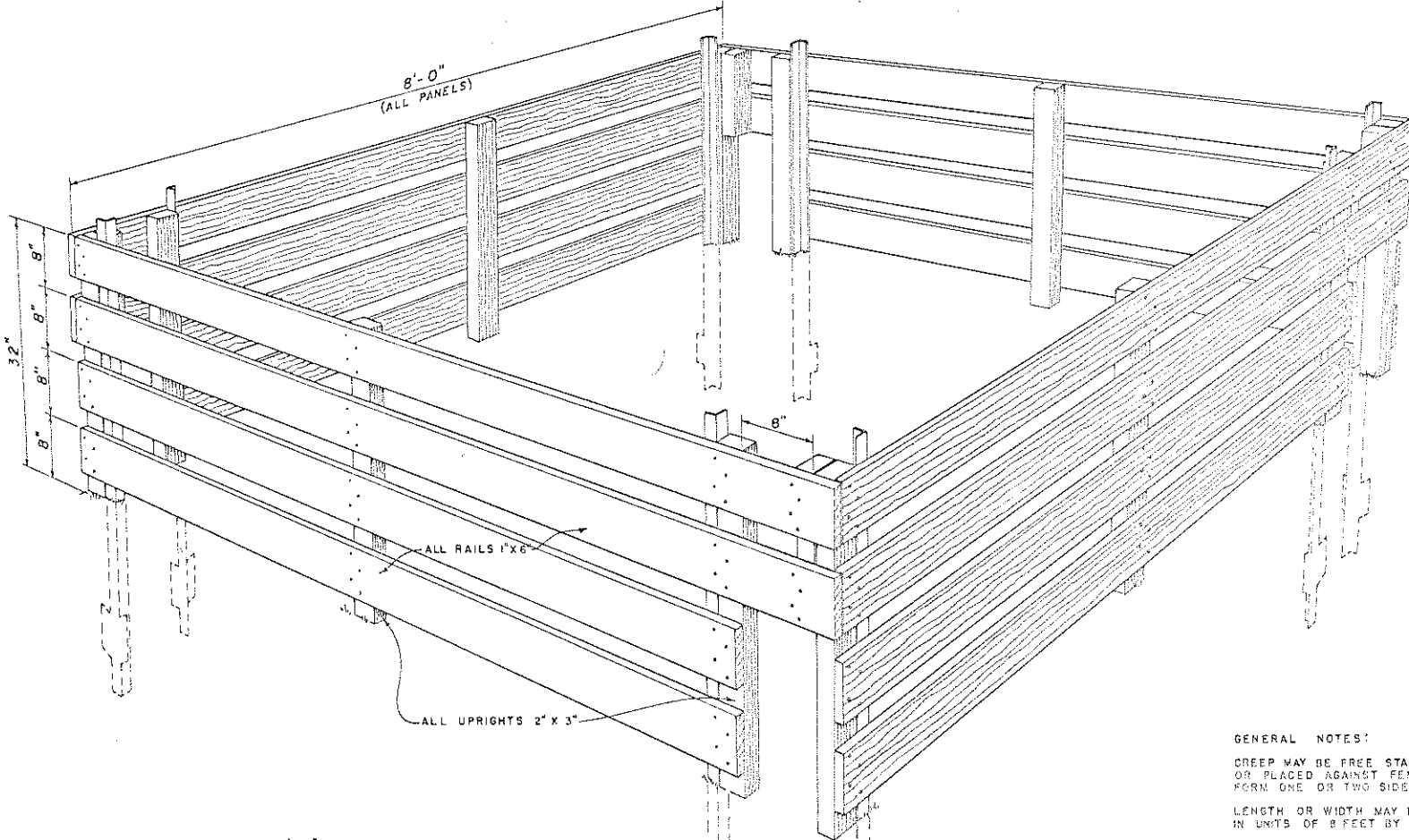
PERSPECTIVE VIEW SHOWING A 4-PANEL CREEP IN FIELD
