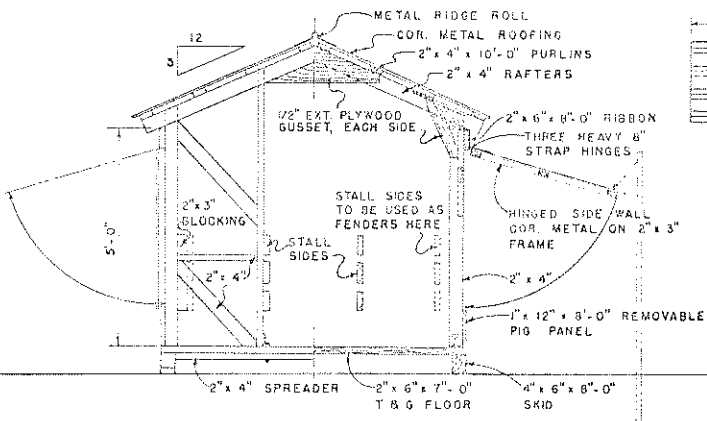
1/2 END FRAMING 1/2 CROSS SECTION
