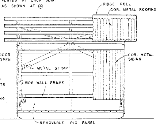
SIDE ELEVATION CUT AWAY TO SHOW FRAMING
