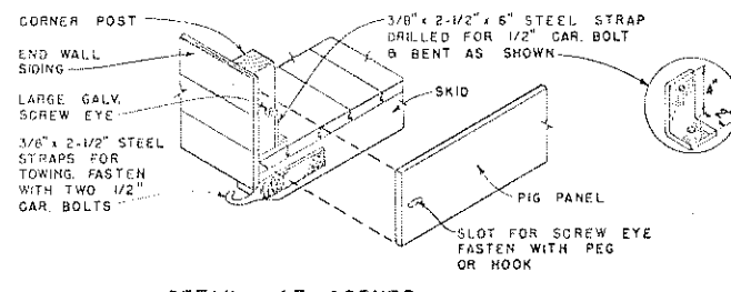
DETAIL AT CORNER
