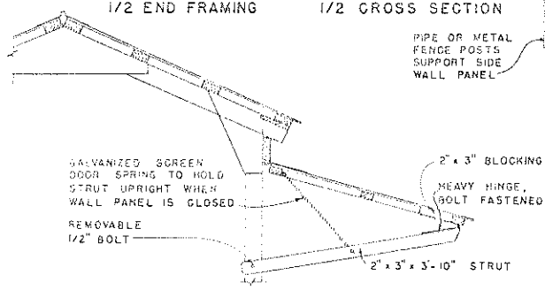
ALT. SUPPORT FOR WALL PANELS
