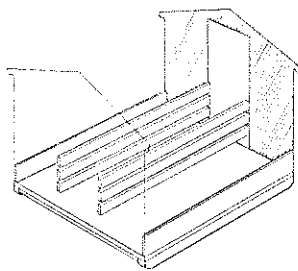
FARROWING STALL FOR SOW & SPACES FOR PIGS DEVELOPING PEN WITH STALL SIDES USED AS FENDERS FOR SHADE PANELS OUT, SIDES & DOORS OPEN DIAGRAMS SHOWING VARIOUS USES OF BUILDING
