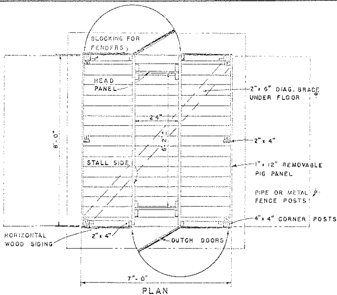
FARROWING STALL FOR SOW & SPACES FOR PIGS DEVELOPING PEN WITH STALL SIDES USED AS FENDERS FOR SHADE PANELS OUT, SIDES & DOORS OPEN DIAGRAMS SHOWING VARIOUS USES OF BUILDING
