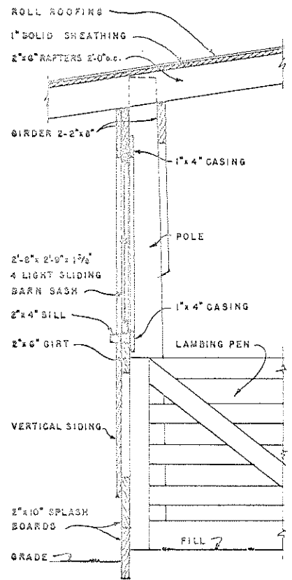
SECTION THRU REAR WALL
