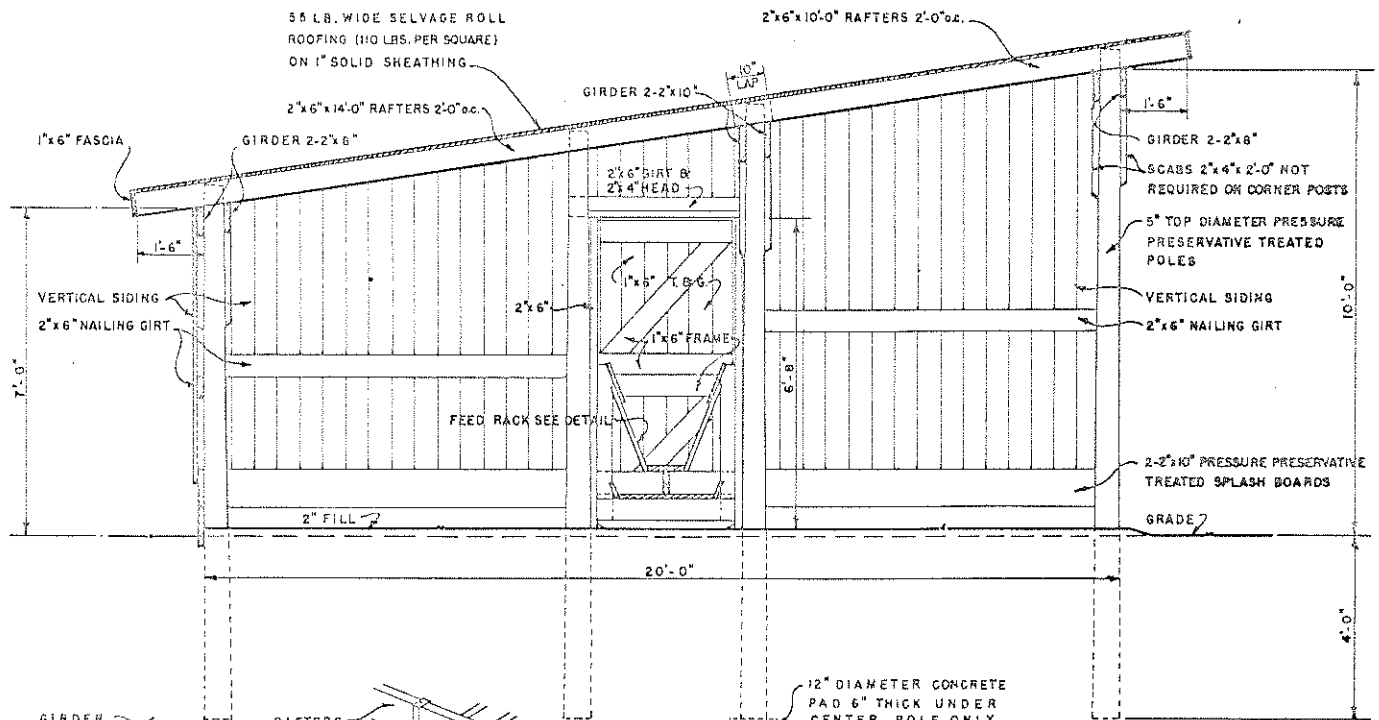
SECTION B-B
