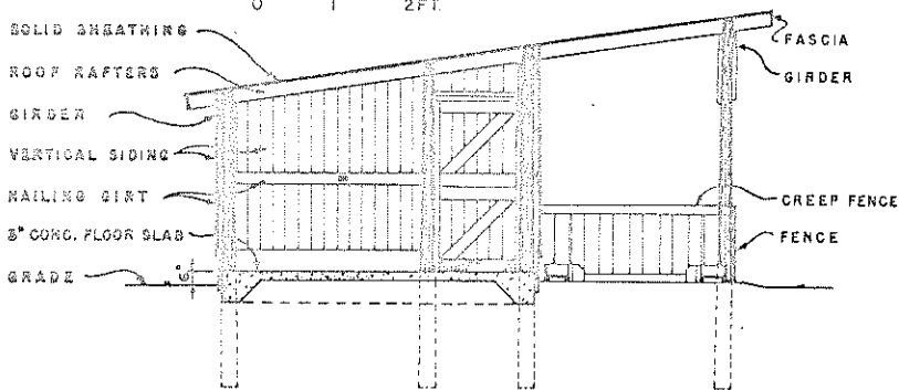
RATPROOFING OF FEED ROOM
