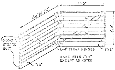
HINGED PANELS FOR TEMPORARY LAMBING PENS
