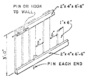
CREEP FENCE
