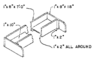
LAMB FEED TROUGH
