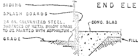
RATPROOFING OF FEED ROOM
