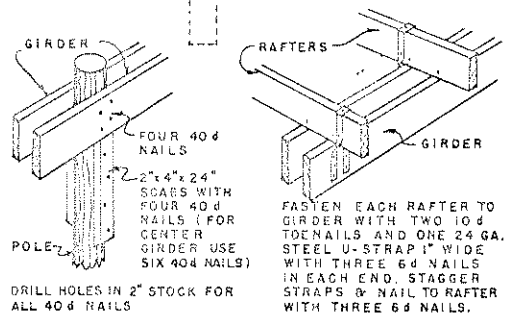
NAILING DETAIL NO SCALE
