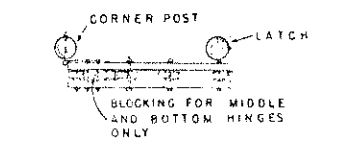
SECTIONAL PLAN AT "C-C"
