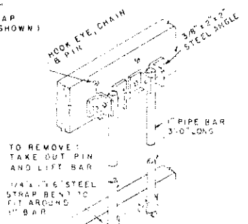
REMOVABLE SIDE BARS
