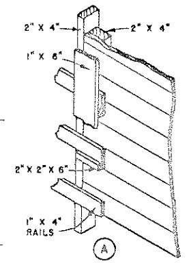
PANEL DETAIL AT CORNER OF BUILDING 0 1 2 FT.
