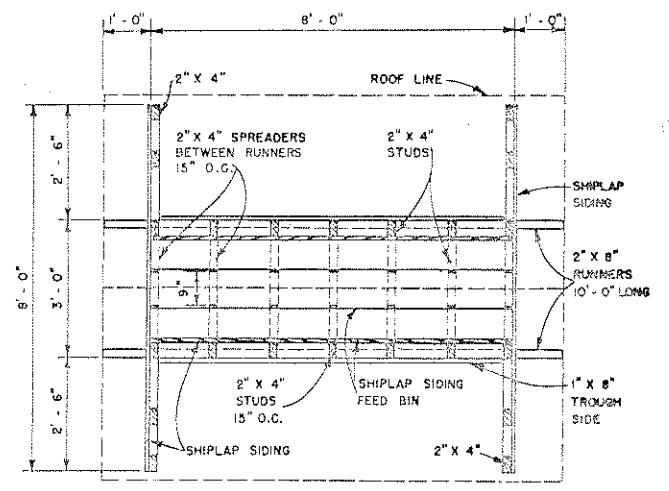
PLAN A-A 0 1 2 3 FT.
