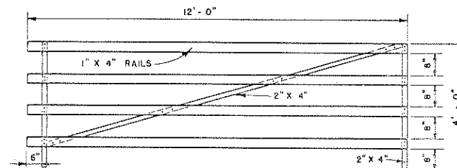
MOVABLE SIDE FENCE PANEL
