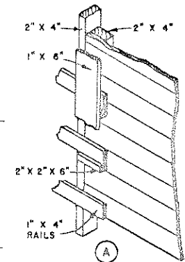
PANEL DETAIL AT CORNER OF BUILDING
