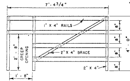
MOVABLE END FENCE PANEL
