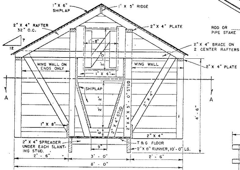
SECTION THROUGH SELF-FEEDER 0 1 2 FT.
