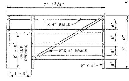
MOVABLE END FENCE PANEL 0 1 2 3 FT.
