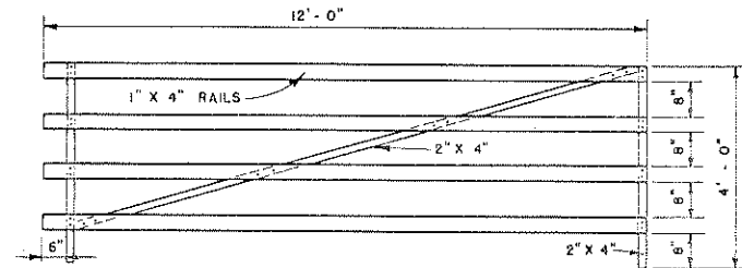
MOVABLE SIDE FENCE PANEL 0 1 2 3 FT.
