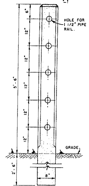
DETAIL OF CONCRETE POSTS SCALE: 0 1 FT.
