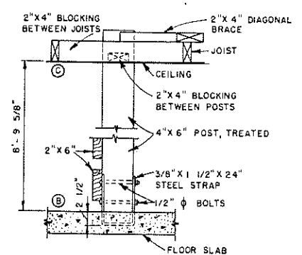
POST DETAIL SCALE: 0 1 FT.
