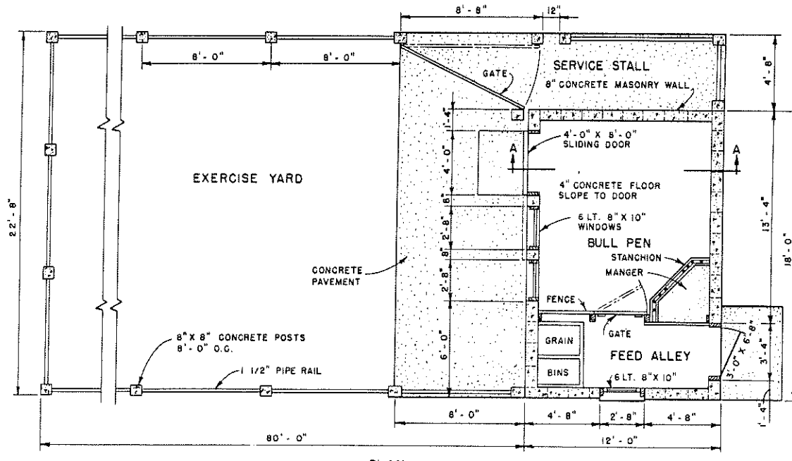
PLAN SCALE: 0 2 4 6 FT.
