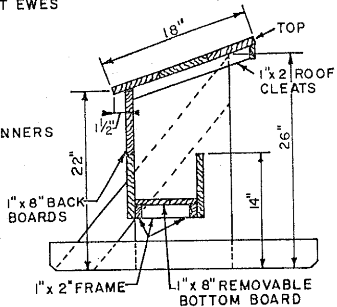
CROSS SECTION
