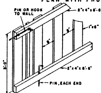
CREEP FENCE
