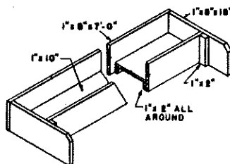
LAMB FEED TROUGH
