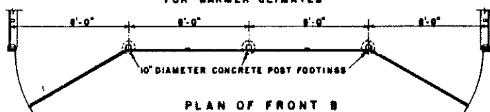
PLAN OF FRONT B
