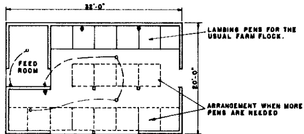
PLAN SHOWING LAMBING PEN ARRANGEMENT NO SCALE
