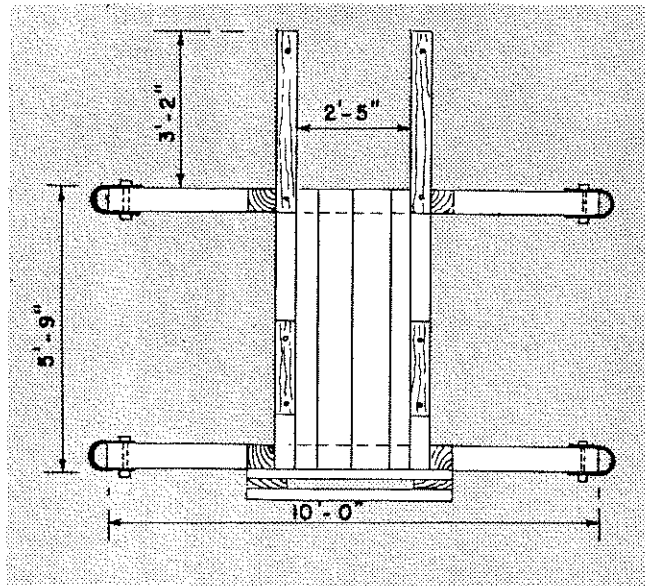
PLAN VIEW
