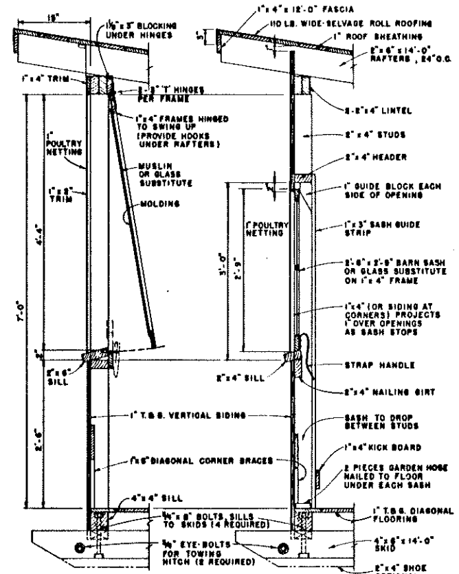
SECTION A-A ALTERNATE FRONT
