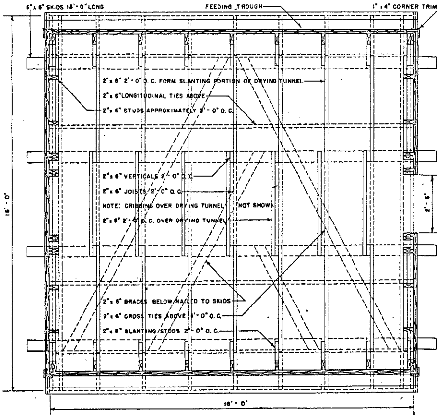
PLAN SCALE - \frac{3}{8} \"/>
