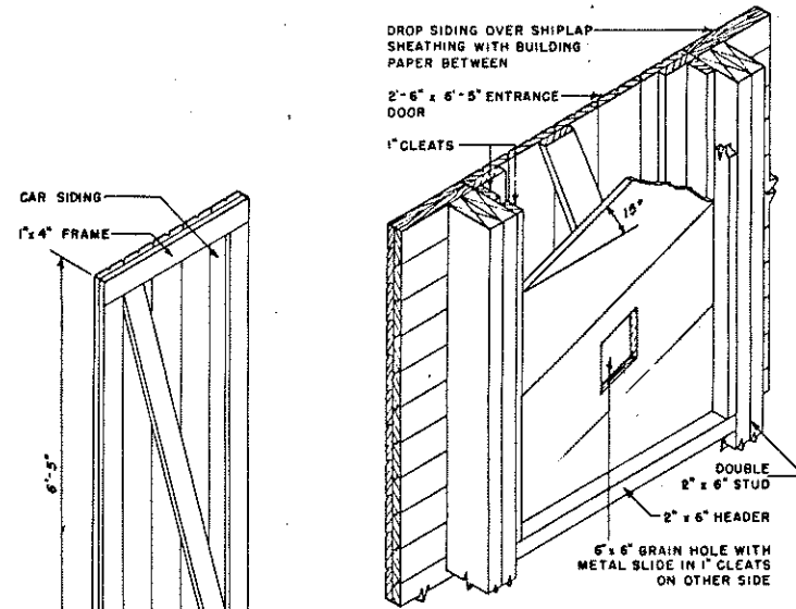
DETAIL AT ENTRANCE DOOR NOT TO SCALE
