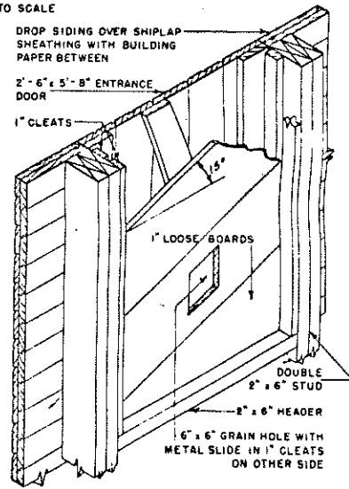
DETAIL AT DOOR NOT TO SCALE
