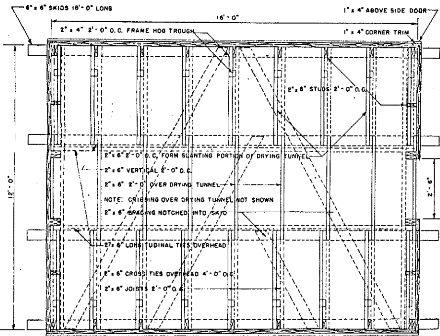
PLAN SCALE - \frac{3}{8} " = 1'-0"
