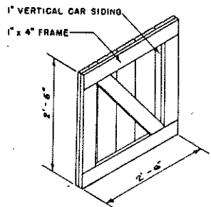
FILLING DOOR NOT TO SCALE
