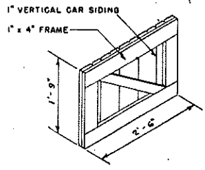
TUNNEL DOOR NOT TO SCALE
