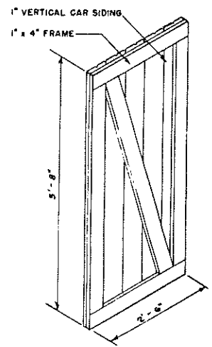
ENTRANCE DOOR NOT TO SCALE
