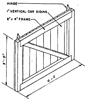
SIDE DOOR NOT TO SCALE
