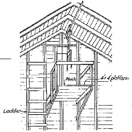
HAY FORK SERVICE PLATFORM
