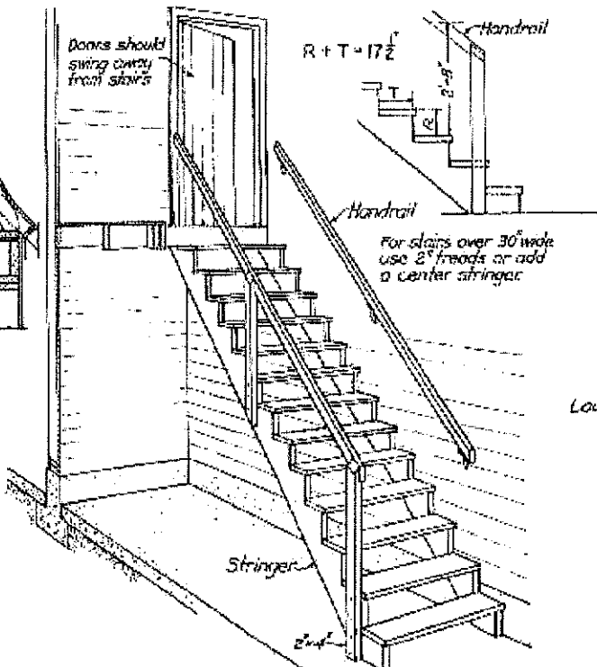
SAFE STAIR CONSTRUCTION
