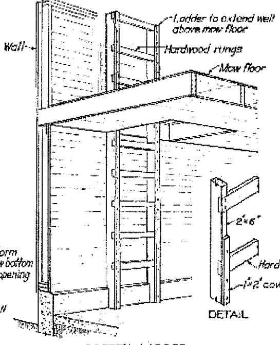
SAFETY LADDER
