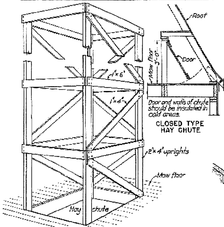
HAY CHUTE GUARD
