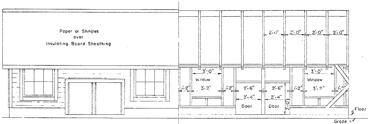
ELEVATION (Southern Exposure)
